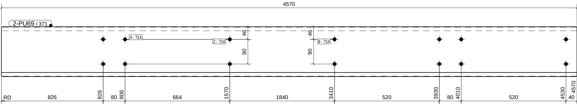
FRONT VIEW
